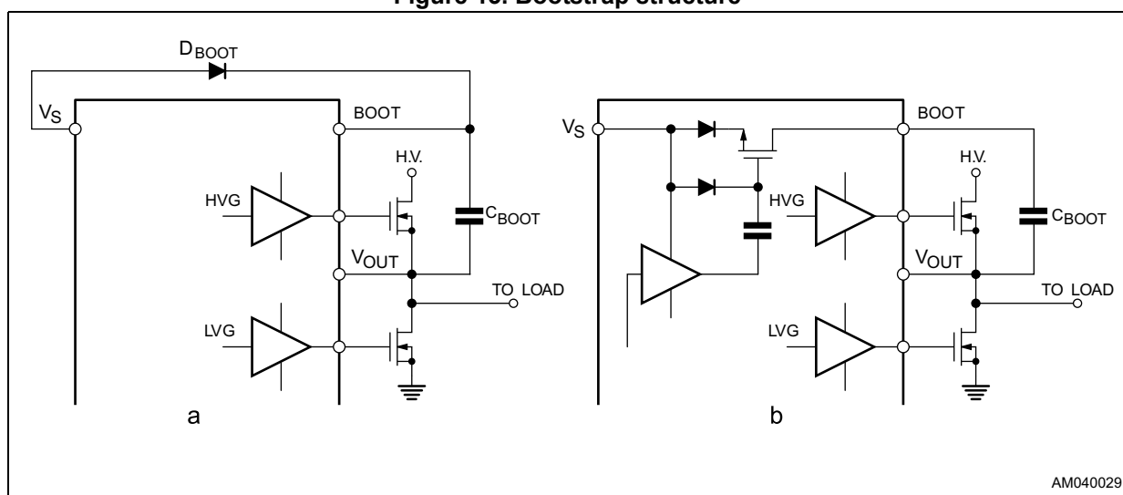
Figure 13. Bootstrap structure
