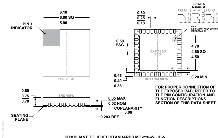
Figure 73. 40-Lead Lead Frame Chip Scale Package [LFCSP] 6 mm × 6 mm Body and 0.75 mm Package Height (CP-40-7)
