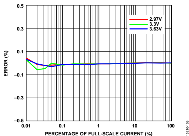
Figure 8. Total Reactive Energy Error as a Percentage of Full-Scale Current over Supply Voltage, Power Factor = 0, T_A = 25^\circ\text{C}
