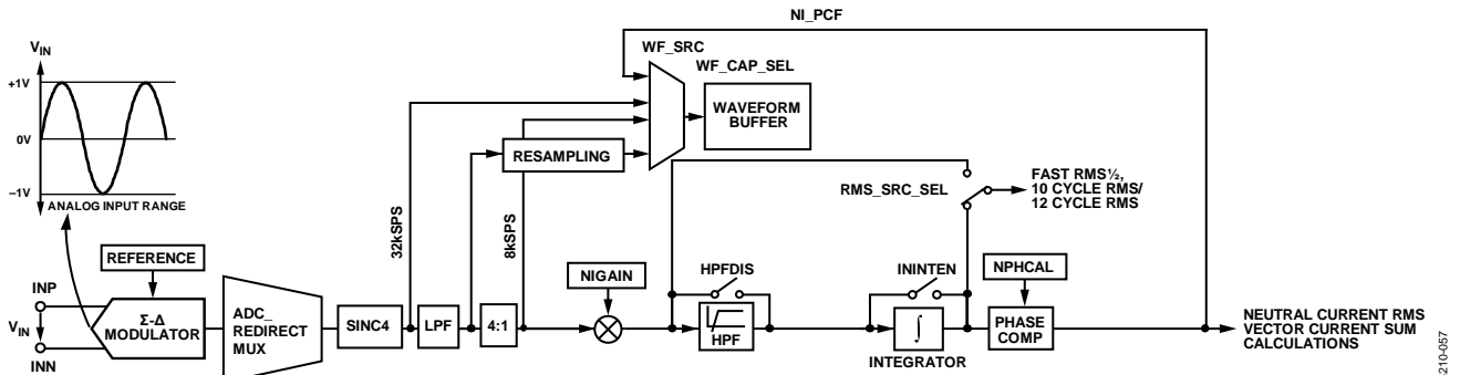
Figure 57. Neutral Current Channel (IN) Datapath
