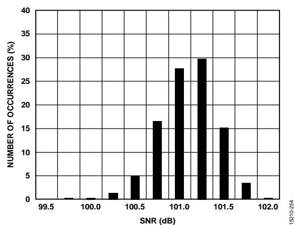
Figure 54. SNR Histogram of ADC SNR for 1000 Devices Tested at T_A = 25^\circ\text{C} with PGA_GAIN = 1 and 8 kSPS Data Rate
