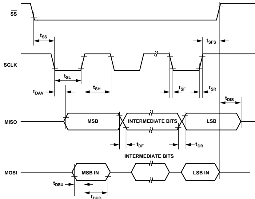
Figure 2. SPI Interface Timing Digram
