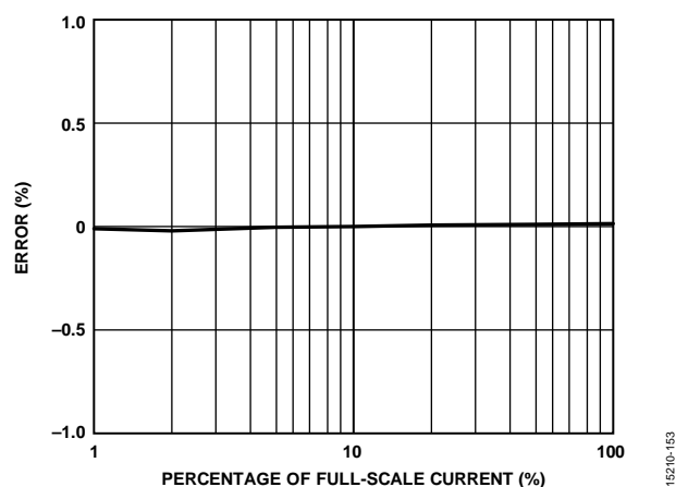
Figure 41. \frac{1}{2} Cycle Current RMS Error, Gain = 4, Integrator On, Data Sourced Before High-Pass Filter and Calibrated for Offset, Register CONFIG0, Bit RMS_SRC_SEL = 1
