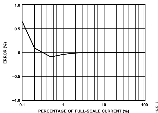
Figure 40. \frac{1}{2} Cycle Current RMS Error, Gain = 4, Integrator On, Data Sourced After High-Pass Filter, Register CONFIG0, Bit RMS_SRC_SEL = 0
