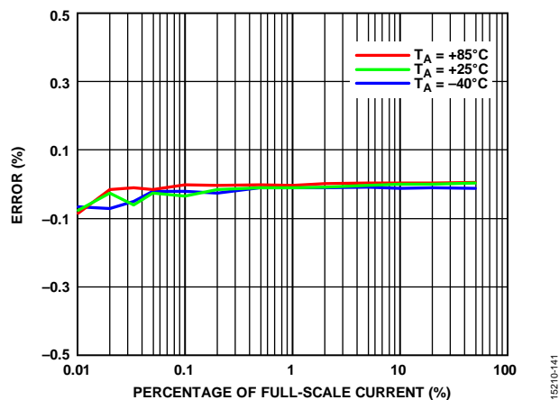
Figure 10. Fundamental Active Energy Error as a Percentage of Full-Scale Current over Temperature, Power Factor = 1
