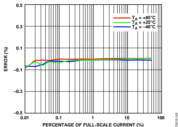
Figure 12. Fundamental Apparent Energy Error as a Percentage of Full-Scale Current over Temperature, Power Factor = 1
