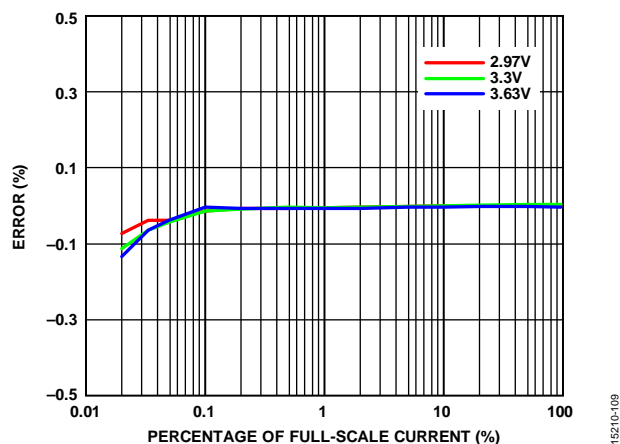
Figure 9. Total Apparent Energy Error as a Percentage of Full-Scale Current over Supply Voltage, Power Factor = 1, T_A = 25^\circ\text{C}
